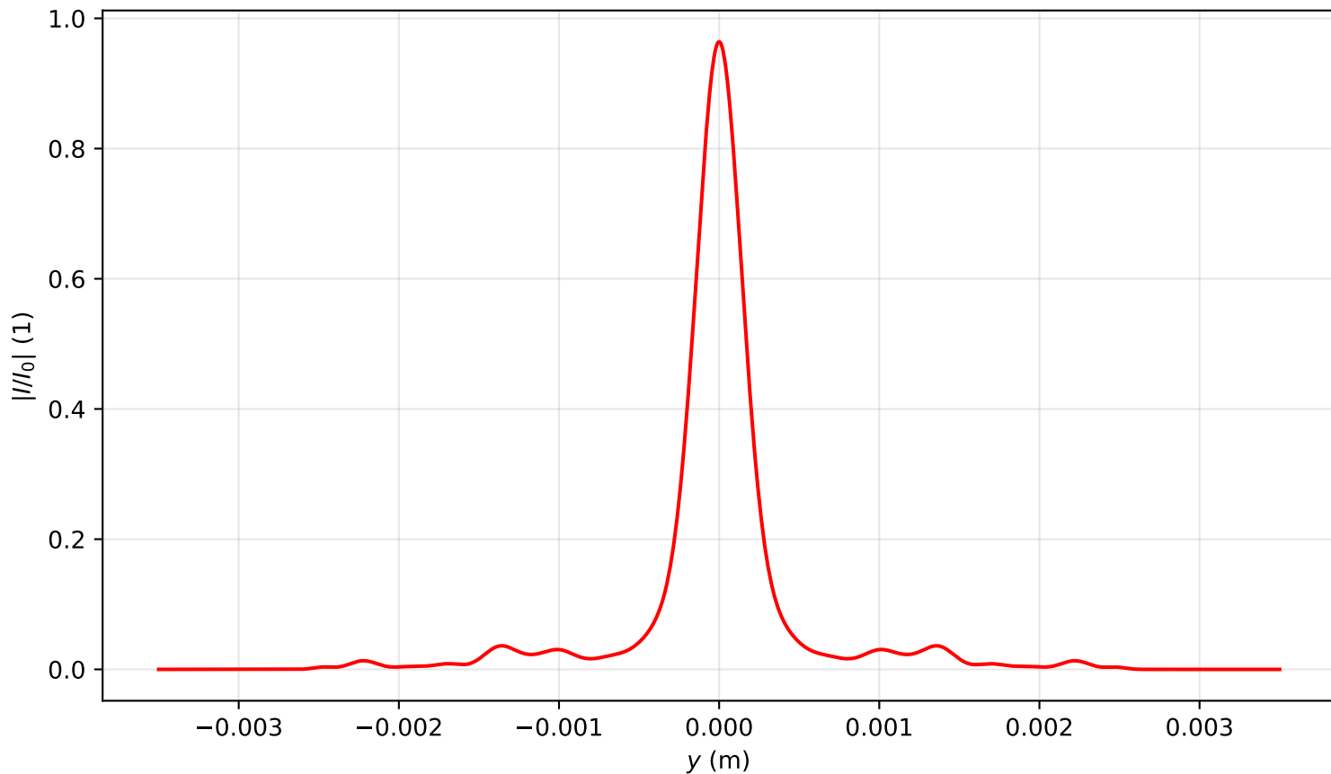
Intensity profile I(x=0, y, z=3.344)/I_0 , P_{in}=4.5P_{cr} , artificial time
